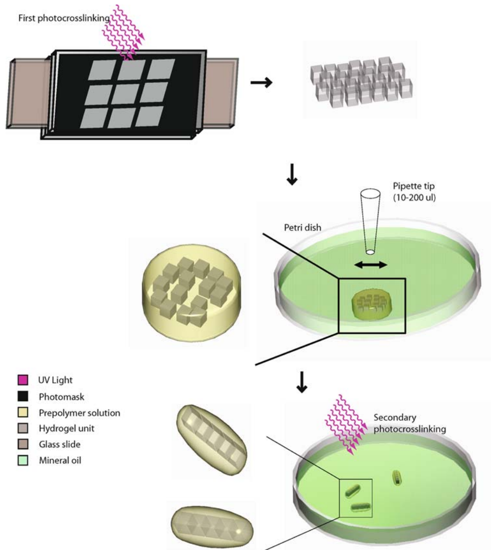
FIGURE 1. Schematic representation of the microgel assembly process: shape-controlled microgels are synthesized by photolithography; the microgels are then transferred into a petri dish filled with mineral oil; mechanical agitation is applied through manual movement of a pipette-tip to facilitate the microgel assembly formation; microgel assemblies are stabilized by a secondary cross-linking.
