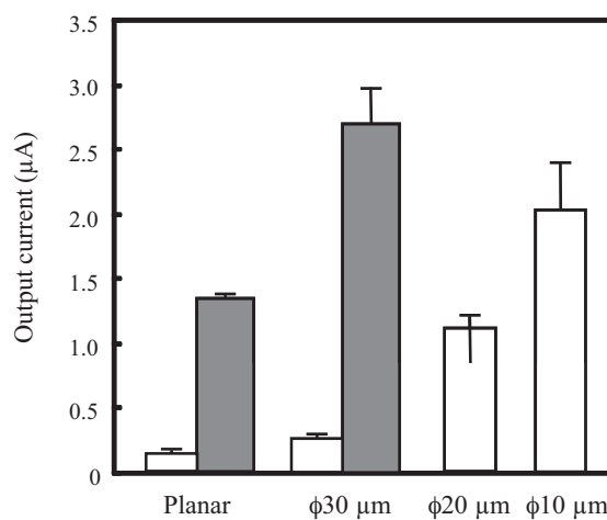
Fig. 4. Effects of dimensions of the micropillar electrodes and the modification with gold-black on oxidation current of L-ascorbic acid. Gray column, with gold-black; white column, without gold-black. The error bars indicate standard deviation (SD) calculated from at least three independent experiments for each plot.
