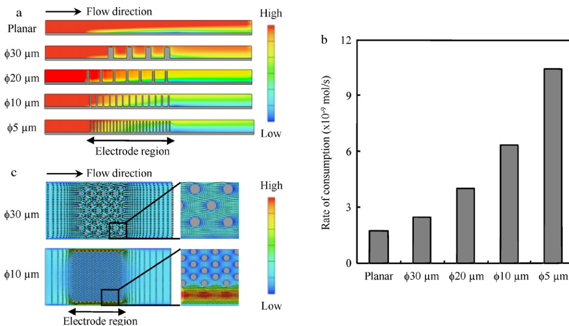
Fig. 2. Calculated results of concentration and flow velocity distributions around the 3D micropillar electrodes. (a) Distribution of the concentration of L-ascorbic acid in the central cross section along the microchannel (side view). The solution flows from the left to the right, and L-ascorbic acid is oxidized and consumed at the electrode. Lower concentrations of L-ascorbic acid are shown in blue. (b) Rate of consumption of L-ascorbic acid calculated from the mass balance between the inlet and outlet. (c) Distribution of flow velocity in the horizontal cross section at the middle height of the microchannel (top view). The magnified views show the flow streams between the micropillars and the lateral walls of the microchannel. The solution flows from the left to the right and is disturbed by the 3D electrode. Higher velocities are shown in red. The microchannel was 500 \mu\text{m} in width and 55 \mu\text{m} in height. The dimensions of the micropillar electrodes are listed in Table 1. (For interpretation of the references to color in this figure legend, the reader is referred to the web version of the article.)
