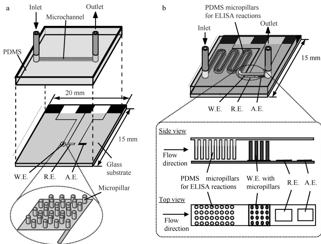
Fig. 1. Schematic of microdevice containing 3D micropillar electrodes and a microchannel. (a) Device used to characterize the 3D electrodes with L -ascorbic acid in numerical simulation and experiments. (b) Device used for electrochemical ELISA. Reactions for ELISA were carried out upstream on the surface of the PDMS micropillars and the enzymatically generated electroactive analytes were detected downstream by the micropillar electrodes. W.E., working electrode (Au); R.E., reference electrode (Ag/AgCl); A.E., auxiliary electrode (Au).
