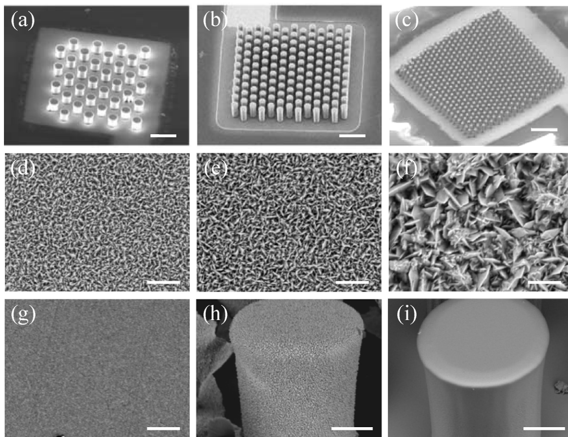
Fig. 3. Scanning electron microscopy images of the working electrodes. (a–c) Micropillar electrodes of \varnothing 30\ \mu\text{m} (a), \varnothing 20\ \mu\text{m} (b), and \varnothing 10\ \mu\text{m} (c). The scale bars are 100\ \mu\text{m} . (d–g) The surface of the planar electrode modified with gold-black at a current density of -30\ \mu\text{A}/\text{mm}^2 (d), -60\ \mu\text{A}/\text{mm}^2 (e), -120\ \mu\text{A}/\text{mm}^2 (f), and an unmodified planar electrode (g). The scale bars are 2.5\ \mu\text{m} . (h and i) Surface of a micropillar of the \varnothing 30\text{-}\mu\text{m} electrode modified with gold-black at -60\ \mu\text{A}/\text{mm}^2 (h) and without modification (i). The scale bars are 10\ \mu\text{m} .
