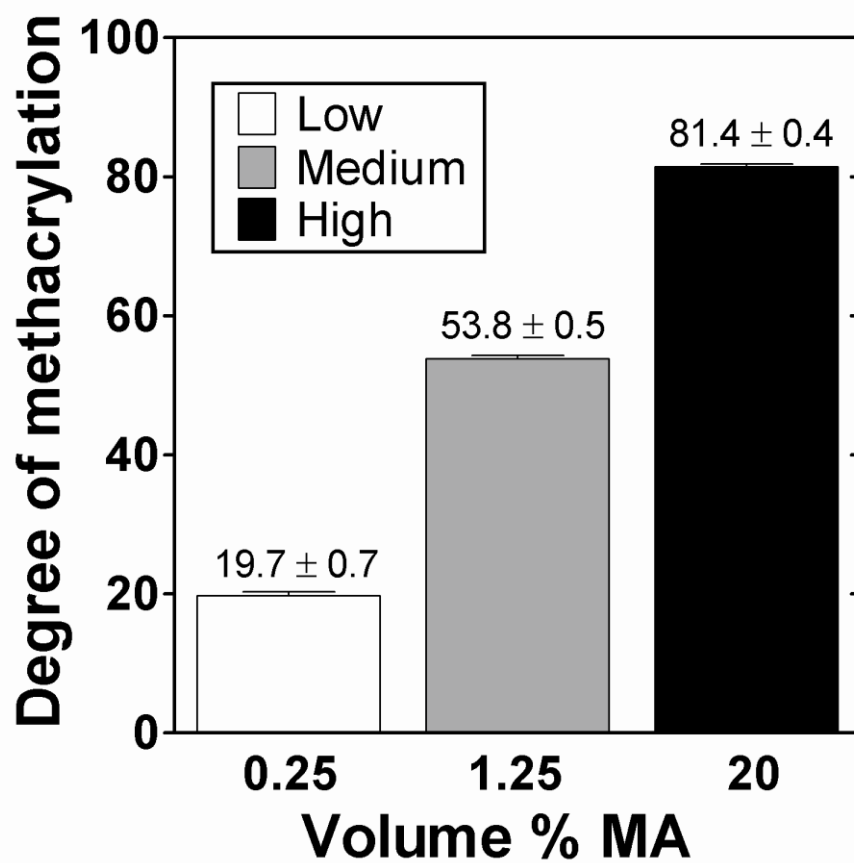
Figure 1. Degree of methacrylation as determined by ^1\text{H-NMR} at various methacrylic anhydride volume percentages present in the synthesis reaction. The number of methacrylate groups incorporated was determined by comparing the integrated intensity of the double bond peak to that of the aromatic side chains. Error bars represent the SD of 3 repeated measurements on each sample.
