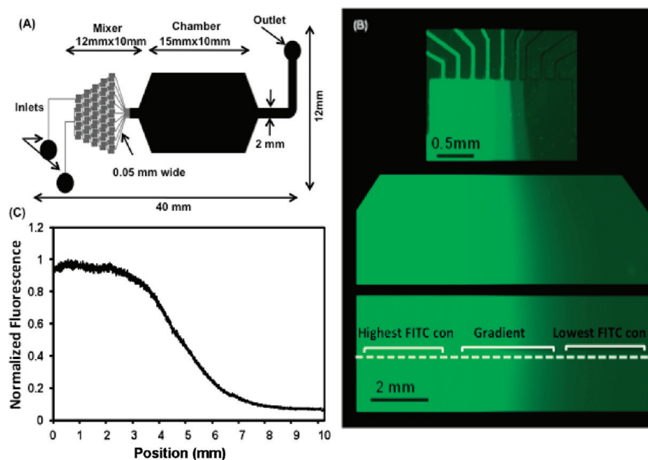
Figure 1. Gradient generation: (A) schematic of the microfluidic device used to generate concentration gradients in a hydrogel with 0.18 mm thickness, (B) fluorescent images of the end of the mixer and the entrance and middle of the chamber where 1 mM FITC-dex solution and water were injected at 0.5 \mu\text{L}/\text{min} through the top and bottom inlets, respectively, (C) gradient profile along the dashed line shown in (B).
