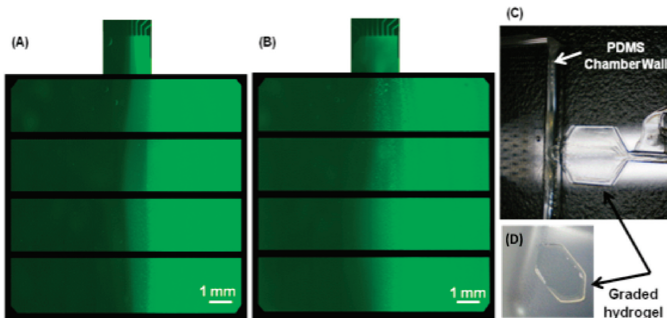
Figure 2. Gradient hydrogel formation: fluorescent images of the FITC-dex concentration gradient in the PEGDA precursor solution (A) before and (B) after UV photopolymerization (the gradients are shown at different regions of the chamber such as the entrance, top, middle, and bottom), (C, D) images of the photopolymerized PEGDA hydrogel loaded with the FITC-dex concentration gradient.
