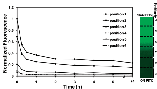
Figure 3. Release profiles from the gradient hydrogels: FITC-dex fluorescence release in PBS from the PEGDA hydrogel loaded with an FITC-dex concentration gradient at different time intervals. The fluorescence intensity values were obtained at different positions along the gradient in the middle of the chamber. Three hydrogels were tested for the release study, and at least three values were measured for each position along the gradient hydrogel. The release profiles were shifted down from position 1 to position 6, confirming that FITC-dex was released from the hydrogel in a gradient manner.
