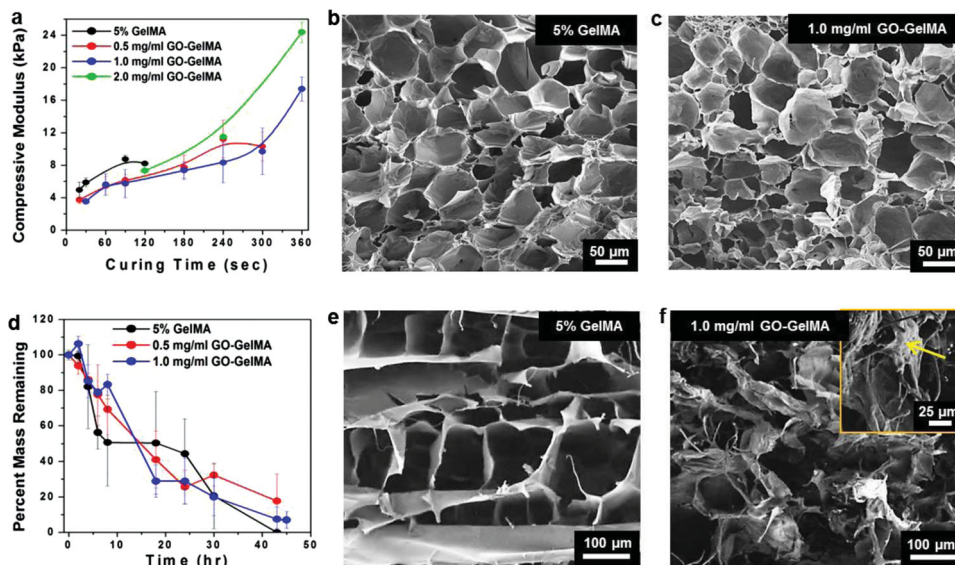
Figure 2. Mechanical, porosity, and degradation characteristics of GO-GelMA hybrid hydrogels. (a) Compressive modulus varies with the GO concentration and UV-exposure time. SEM cross-sectional images of hydrogels with (b) 5% GelMA (0 mg/mL GO, 120 s exposure) and (c) GO-GelMA hybrid (1.0 mg/mL GO, 360 s exposure) reveal similar porosity before collagenase degradation. (d) Degradation profiles of hydrogels with various GO concentrations when exposed to collagenase. SEM cross-sectional images of (e) GelMA and (f) GO-GelMA hydrogels reveal distinctively different gel morphologies after degradation with collagenase for 24 h. In the inset of (f), the yellow arrow indicates a folded GO sheet.
