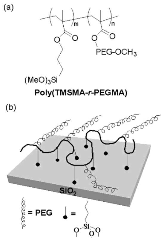
Chart 1. (a) Chemical Structure of the (Trimethoxysilyl)propyl Methacrylate and PEG Methacrylate Random Copolymer, Poly(TMSMA- r -PEGMA) and (b) Schematic Diagram of Self-Assembled Monolayers of the Copolymer on SiO 2 Surface
