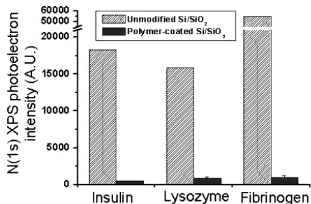
Figure 2. Protein adsorption on control (unmodified) and poly-(TMSMA- r -PEGMA) SAMs on Si/SiO 2 wafer. The relative amount of each protein on the surface is denoted by its N(1s) XPS photoelectron intensity.
